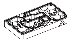
Function plate assembly
