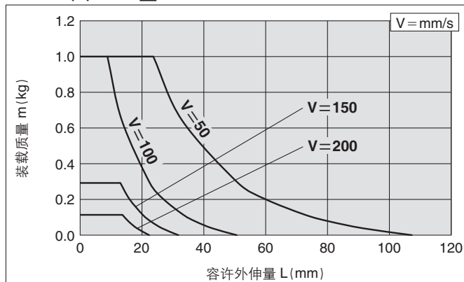
MXQ8 A C -50Z□
