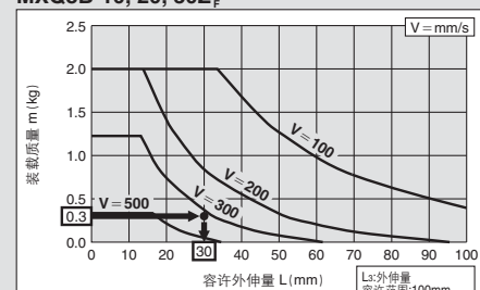
MXQ8B-10, 20, 30Z D
